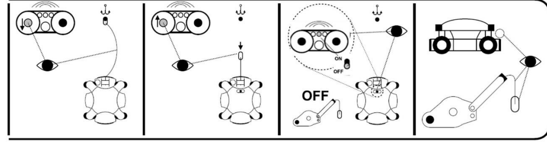
Loosen the winch rope by pushing the drive joystick slightly backward.
