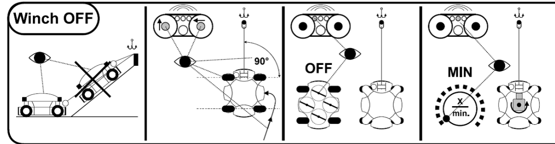
Winch OFF Place the mower at the bottom of the slope
